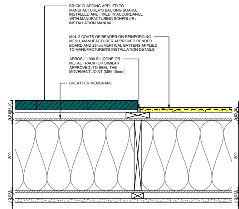
RENDER TO BRICK CLADDING JUNCTION
