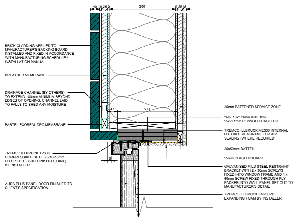
EXTERNAL PANEL DOOR HEADER DETAIL (INWARD OPENING) - BRICK CLADDING (300mm PANEL)
