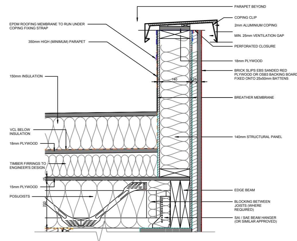
FLAT ROOF DETAIL CLAD PARAPET WALL
